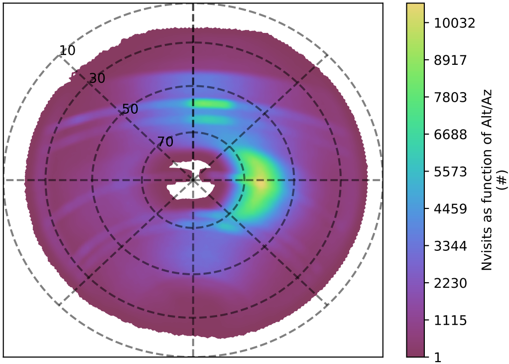
ddf_acor_sf10_ls40_lsr10_v3.4_10yrs all bands: Nvisits as function of Alt/Az
