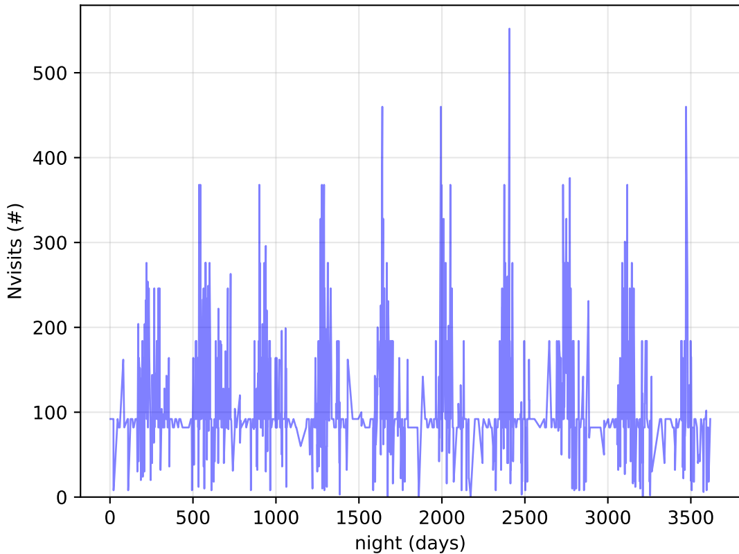
ddf_acor_sf10_ls40_lsr10_v3.4_10yrs DDF: Nvisits
