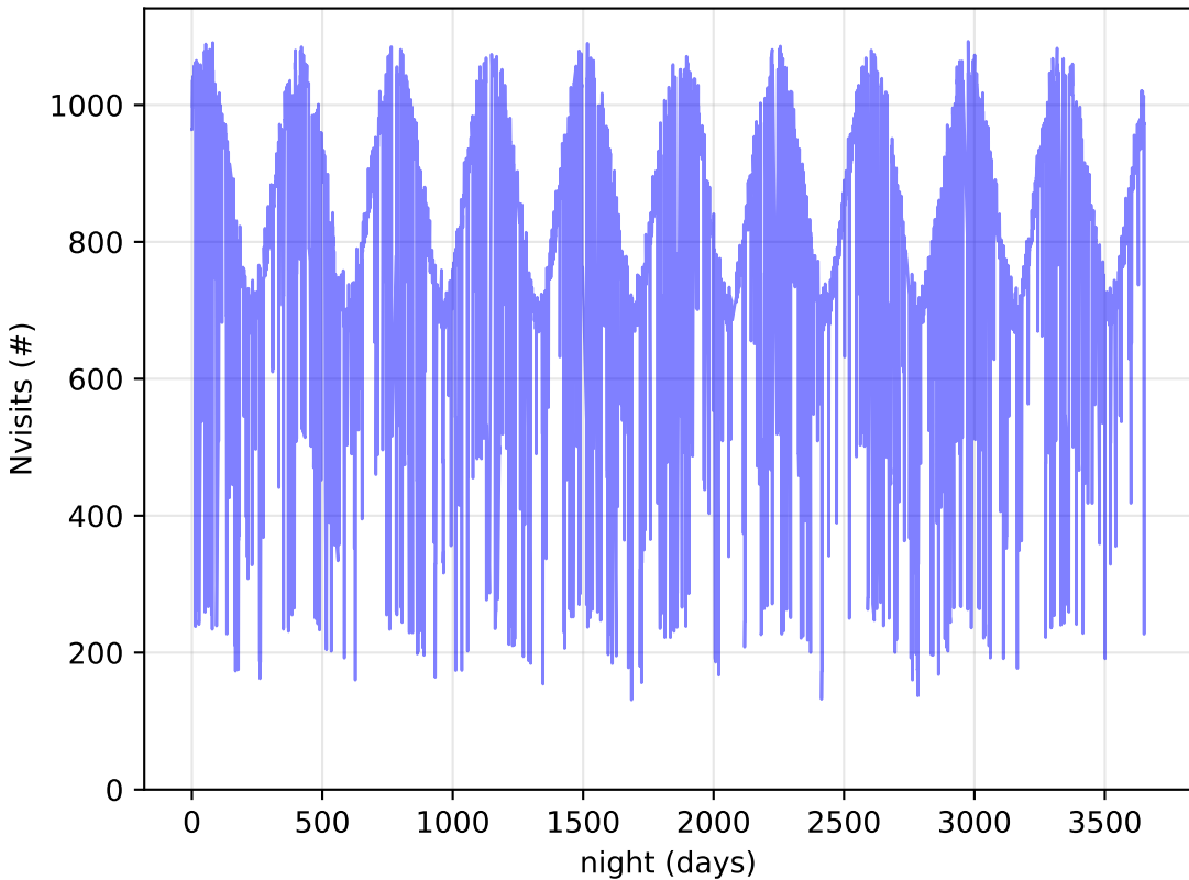
ddf_acor_sf10_ls40_lsr10_v3.4_10yrs All visits: Nvisits
