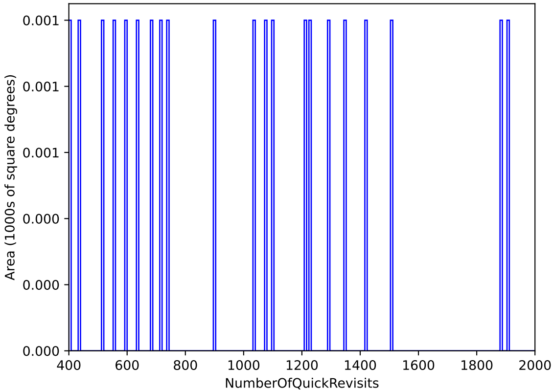
ddf_acor_sf10_lsf40_lsr10_v3.4_10yrs WFD: NumberOfQuickRevisits
