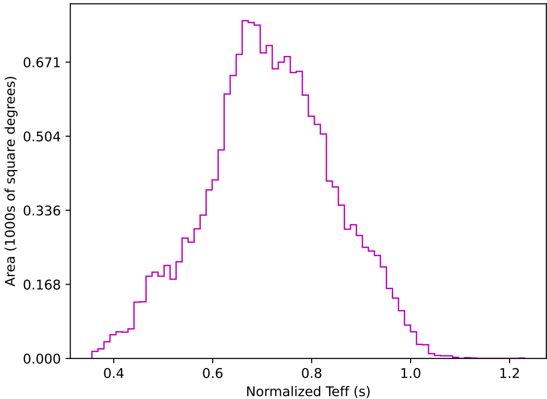
ddf_acor_sf10_lsf40_lsr10_v3.4_10yrs WFD z band: Normalized Teff
