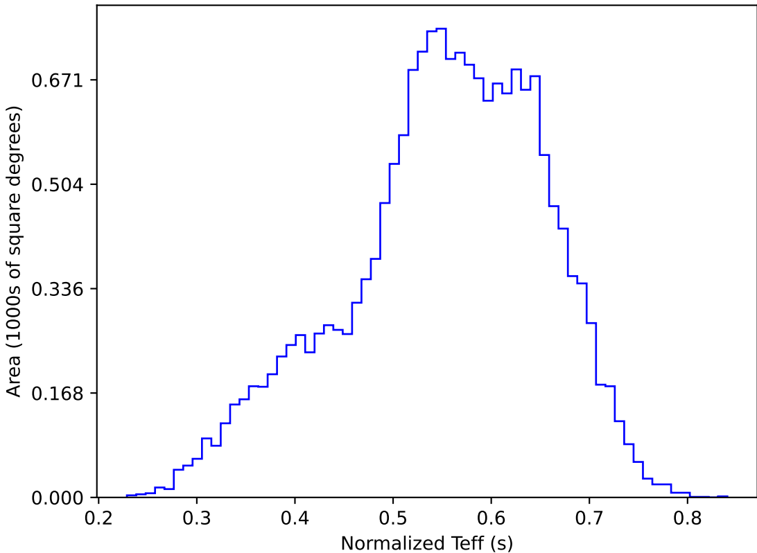
ddf_acor_sf10_lsf40_lsr10_v3.4_10yrs WFD y band: Normalized Teff
