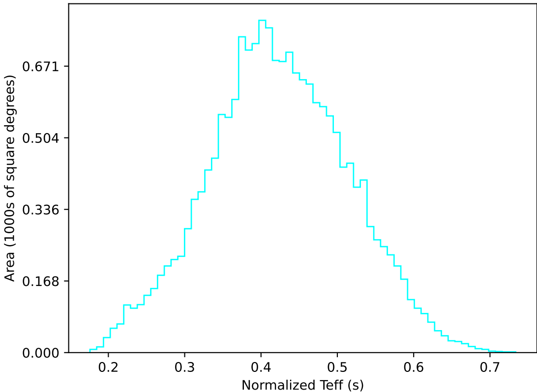
ddf_acor_sf10_lsf40_lsr10_v3.4_10yrs WFD u band: Normalized Teff
