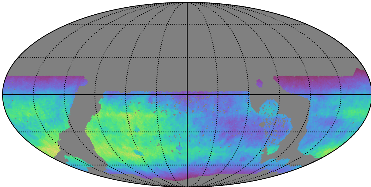
ddf_acor_sf10_lsf40_lsr10_v3.4_10yrs WFD r band: Normalized Teff
