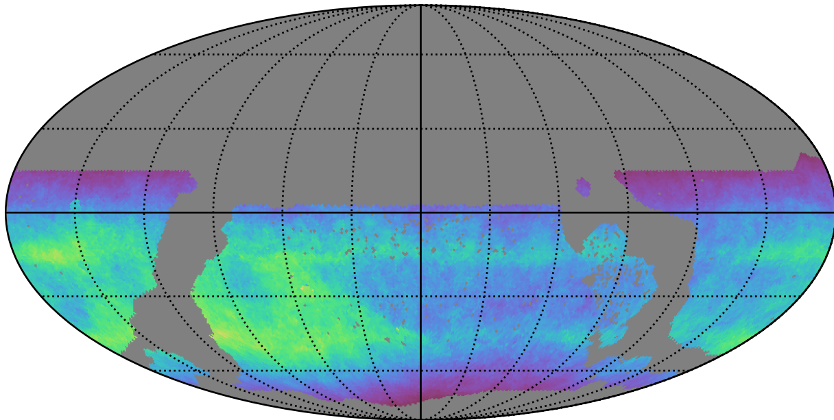
ddf_acor_sf10_lsf40_lsr10_v3.4_10yrs WFD i band: Normalized Teff
