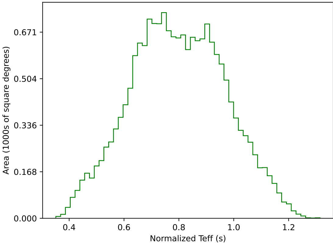
ddf_acor_sf10_lsf40_lsr10_v3.4_10yrs WFD g band: Normalized Teff
