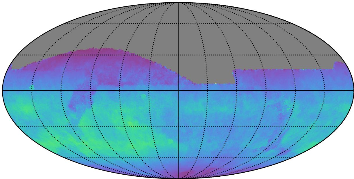
ddf_acor_sf10_lsf40_lsr10_v3.4_10yrs All sky z band: Normalized Teff
