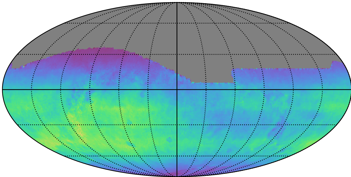
ddf_acor_sf10_lsf40_lsr10_v3.4_10yrs All sky r band: Normalized Teff
