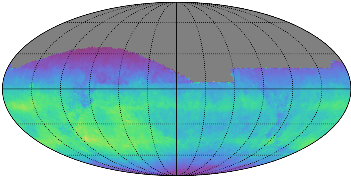
ddf_acor_sf10_lsf40_lsr10_v3.4_10yrs All sky i band: Normalized Teff
