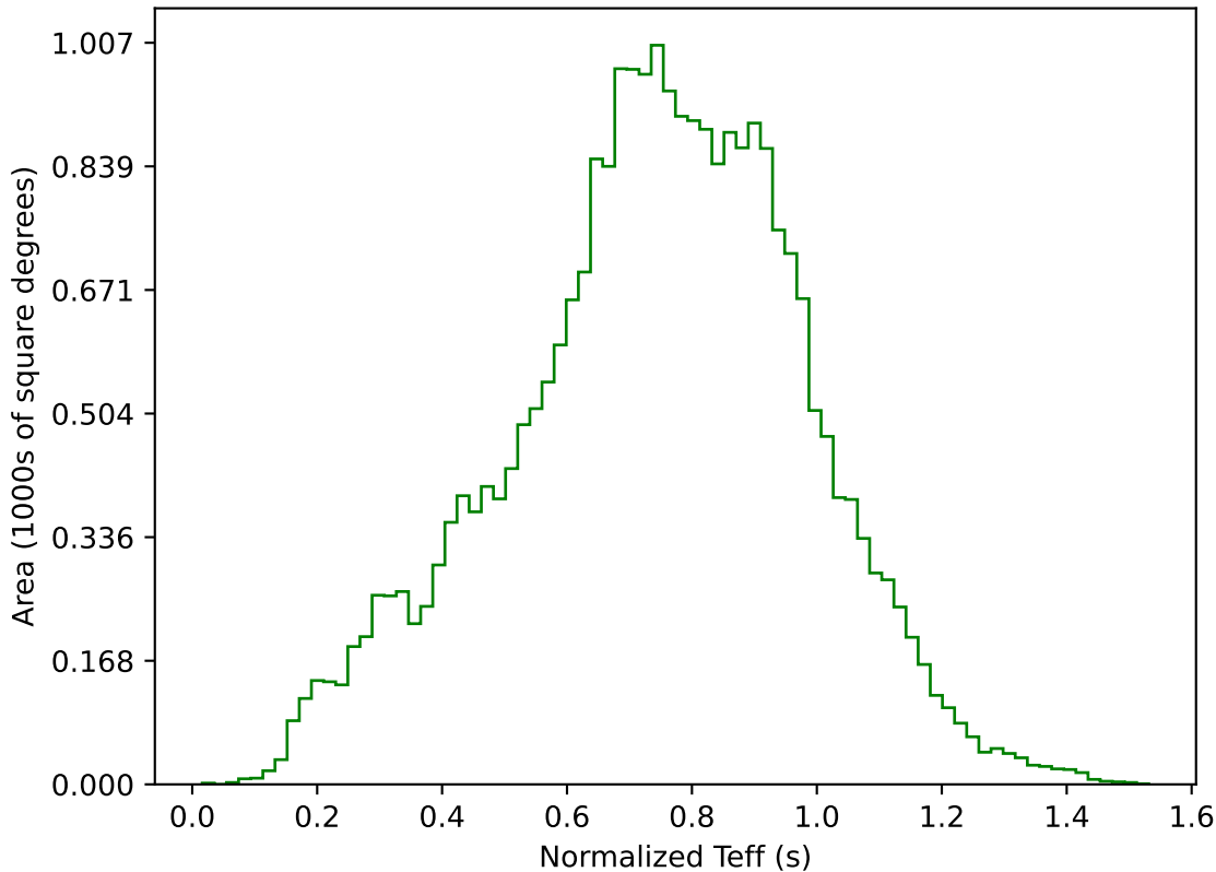
ddf_acor_sf10_lsf40_lsr10_v3.4_10yrs All sky g band: Normalized Teff
