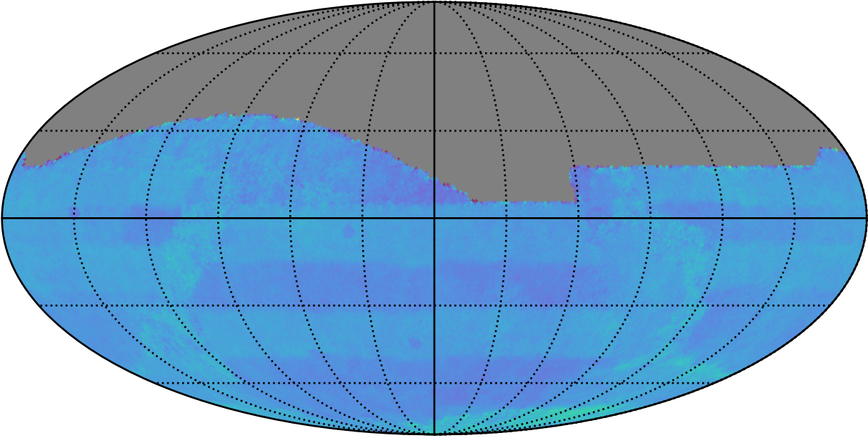
ddf_acor_sf10_lsf40_lsr10_v3.4_10yrs All sky: Normalized Proper Motion Uncert @ 24.0
