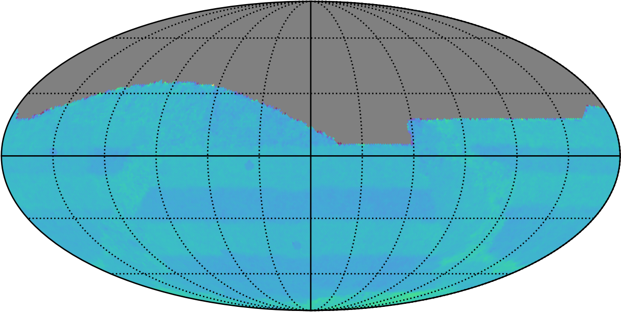
ddf_acor_sf10_lsf40_lsr10_v3.4_10yrs All sky: Normalized Proper Motion Uncert @ 20.5
