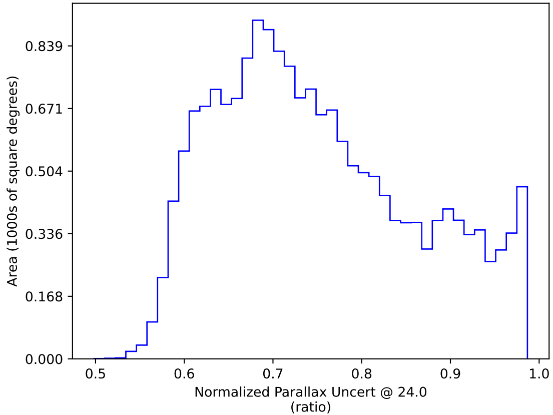
ddf_acor_sf10_lsf40_lsr10_v3.4_10yrs WFD: Normalized Parallax Uncert @ 24.0
