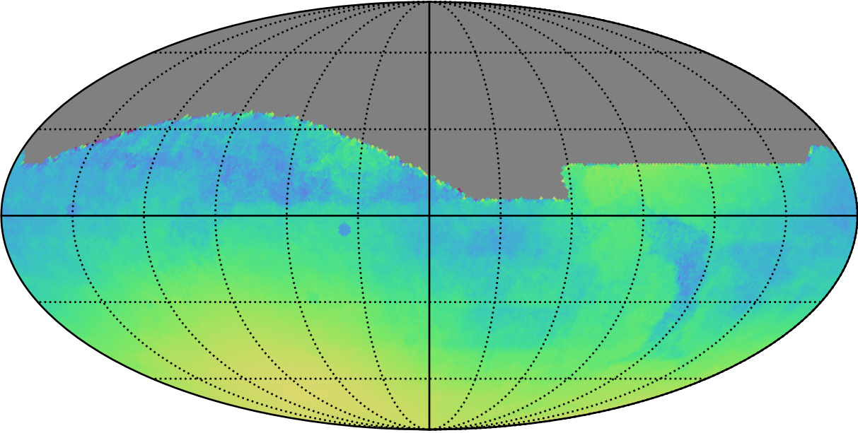
ddf_acor_sf10_lsf40_lsr10_v3.4_10yrs All sky: Normalized Parallax Uncert @ 24.0
