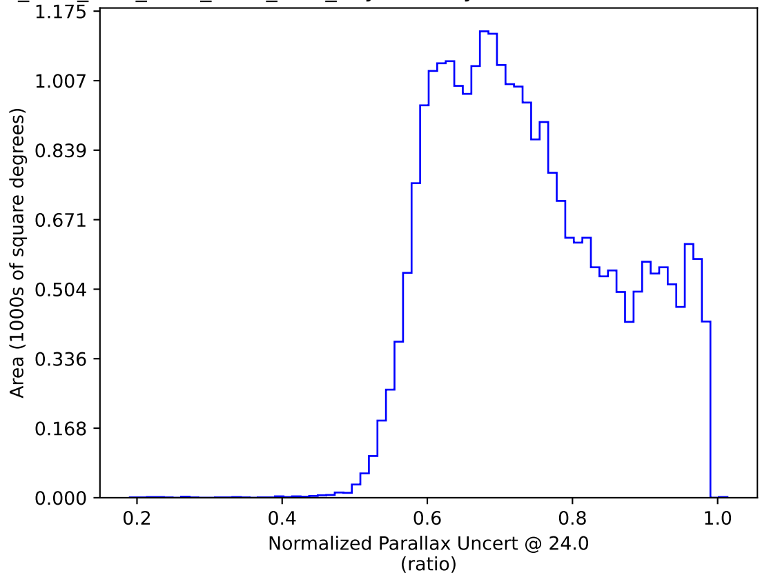
ddf_acor_sf10_lsf40_lsr10_v3.4_10yrs All sky: Normalized Parallax Uncert @ 24.0
