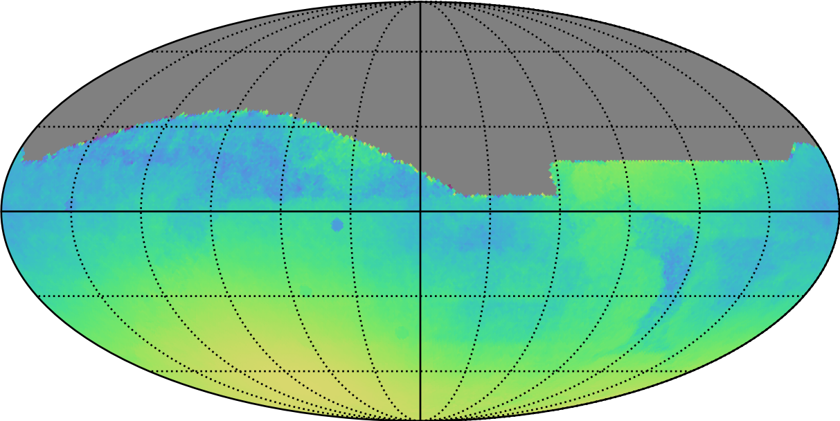
ddf_acor_sf10_lsf40_lsr10_v3.4_10yrs All sky: Normalized Parallax Uncert @ 22.4
