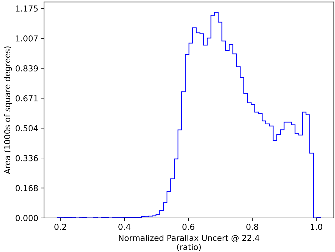
ddf_acor_sf10_lsf40_lsr10_v3.4_10yrs All sky: Normalized Parallax Uncert @ 22.4
