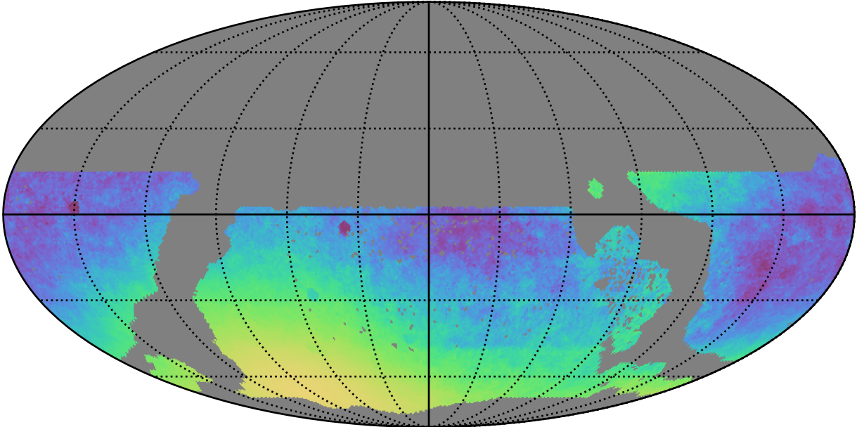
ddf_acor_sf10_lsf40_lsr10_v3.4_10yrs WFD y band only: Normalized Parallax Uncert @ 21.3
