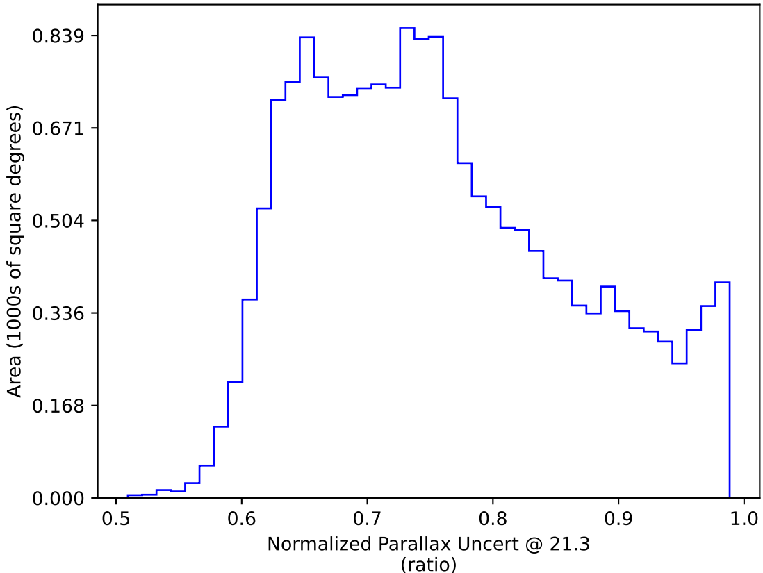
ddf_acor_sf10_lsf40_lsr10_v3.4_10yrs WFD y band only: Normalized Parallax Uncert @ 21.3
