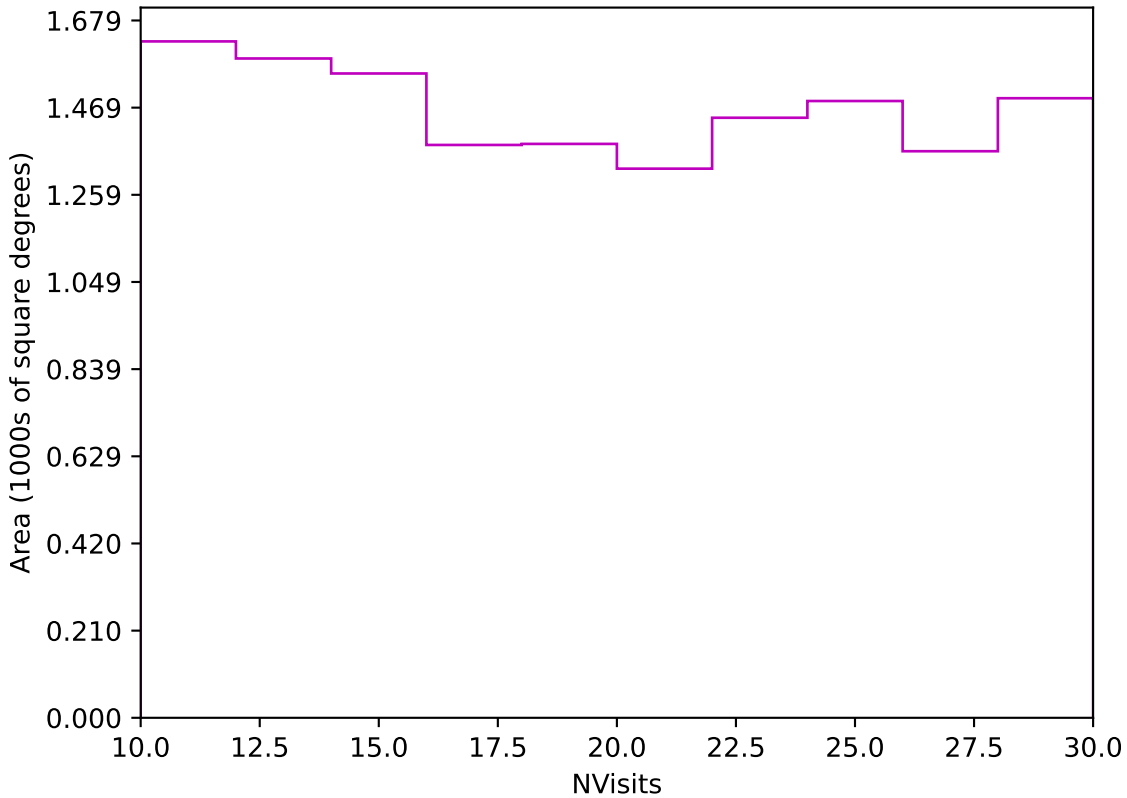
ddf_acor_sf10_lsf40_lsr10_v3.4_10yrs Yr 3-4 z band: NVisits
