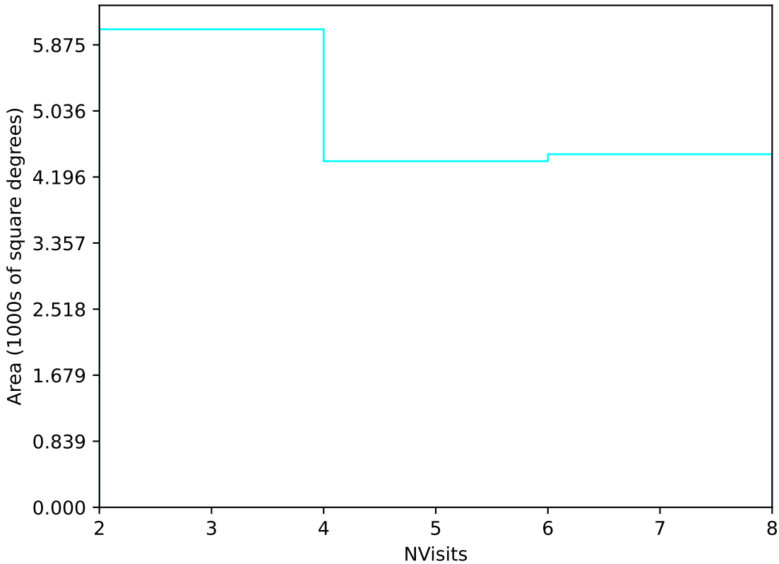
ddf_acor_sf10_lsf40_lsr10_v3.4_10yrs Yr 3-4 u band: NVisits
