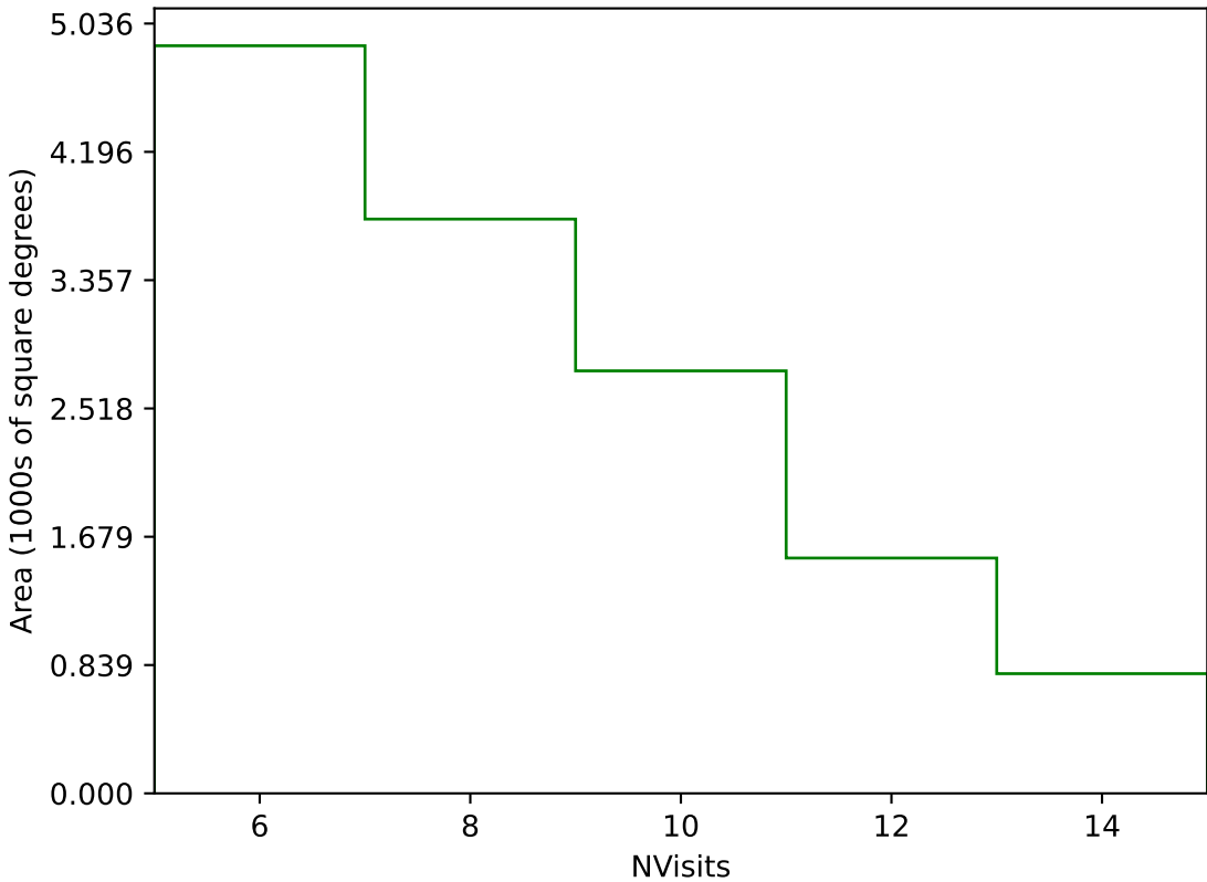
ddf_acor_sf10_lsf40_lsr10_v3.4_10yrs Yr 3-4 g band: NVisits
