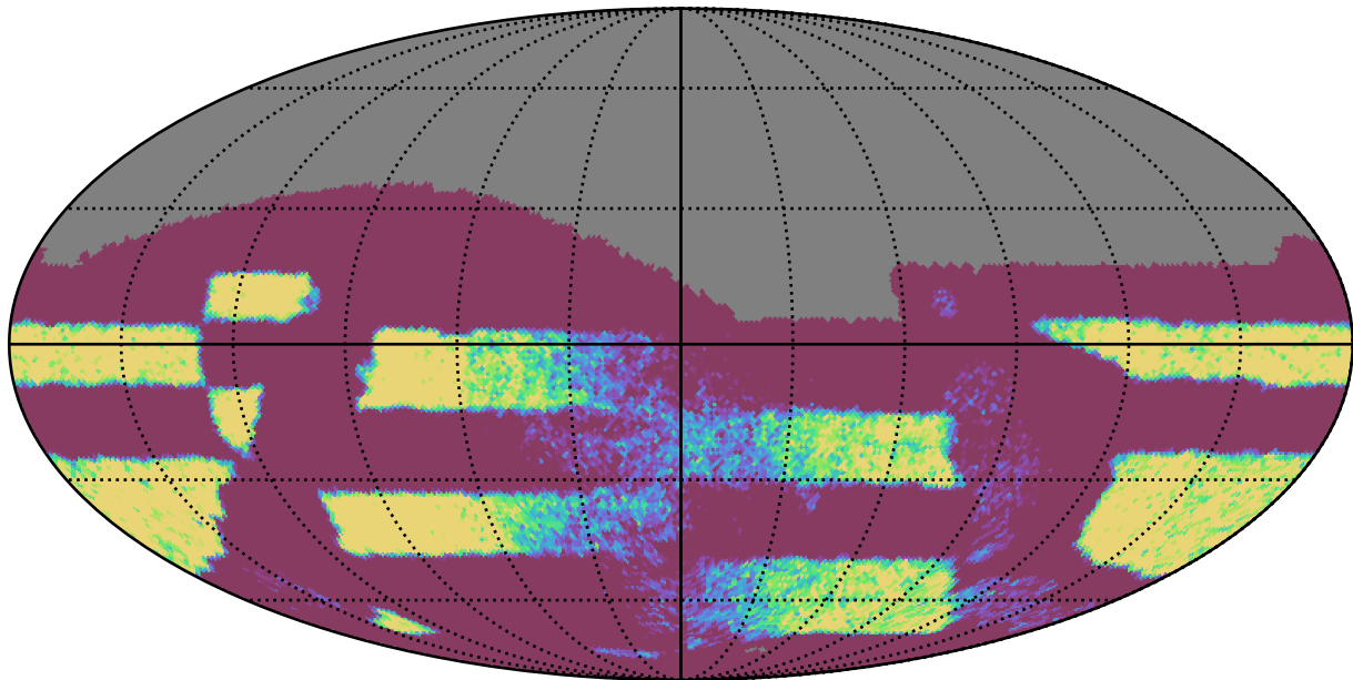
ddf_acor_sf10_lsf40_lsr10_v3.4_10yrs Yr 3-4 all bands: NVisits
