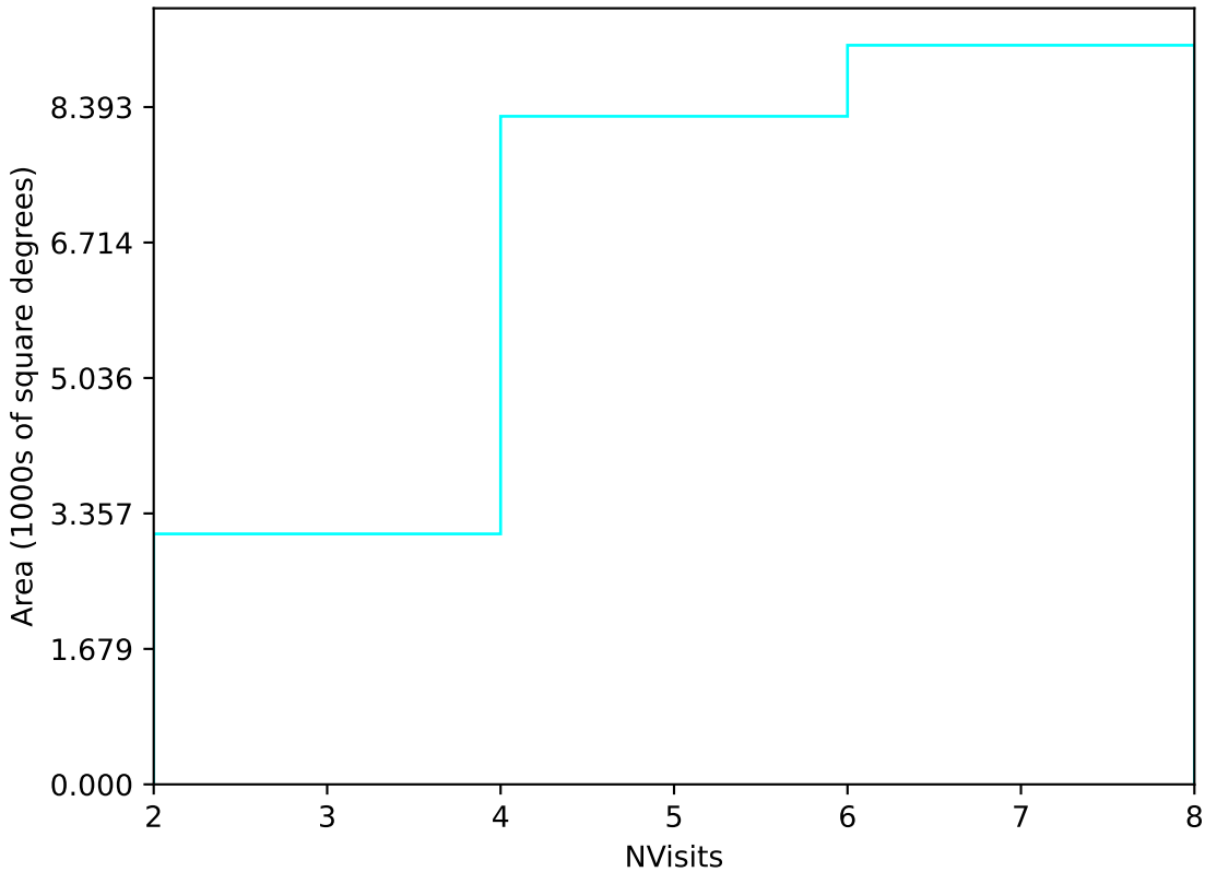
ddf_acor_sf10_lsf40_lsr10_v3.4_10yrs Yr 1 u band: NVisits
