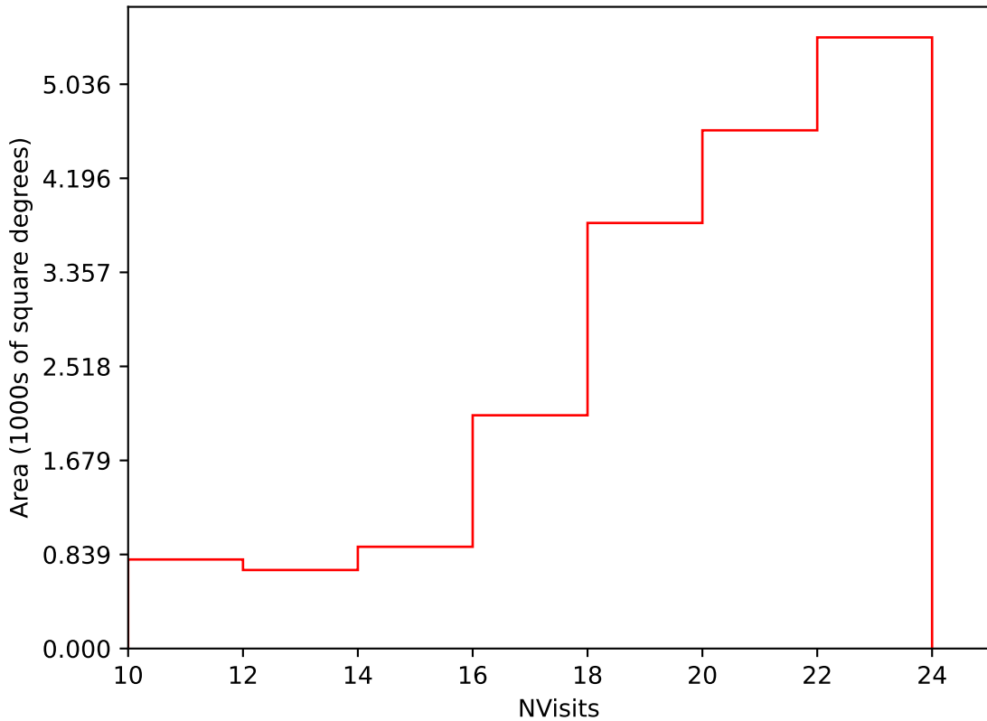
ddf_acor_sf10_lsf40_lsr10_v3.4_10yrs Yr 1 i band: NVisits
