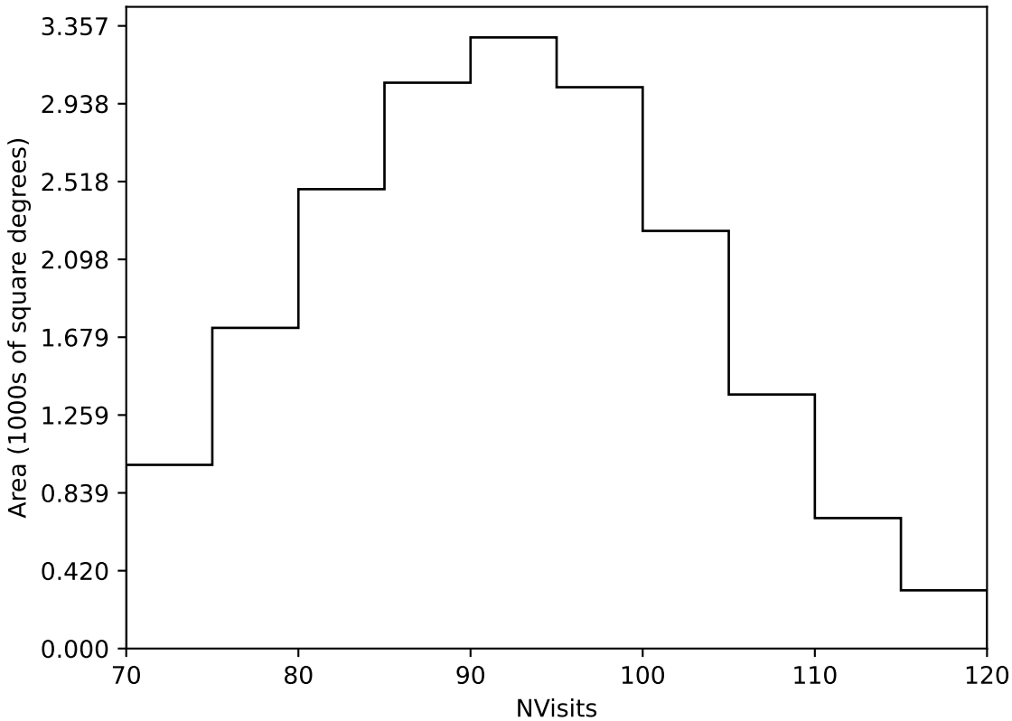
ddf_acor_sf10_lsf40_lsr10_v3.4_10yrs Yr 1 all bands: NVisits
