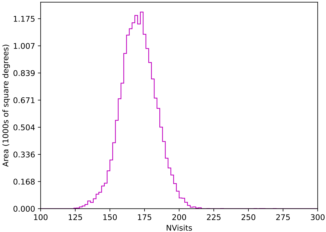
ddf_acor_sf10_lsf40_lsr10_v3.4_10yrs WFD z band: NVisits
