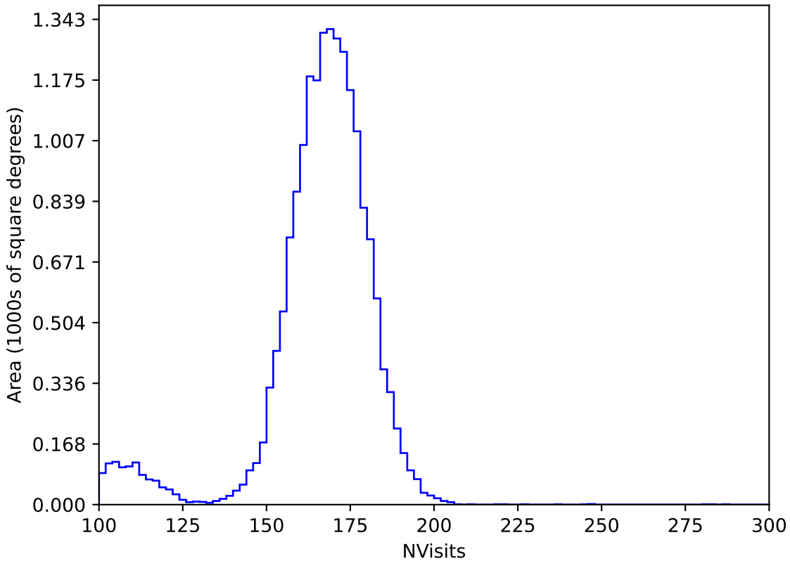
ddf_acor_sf10_lsf40_lsr10_v3.4_10yrs WFD y band: NVisits
