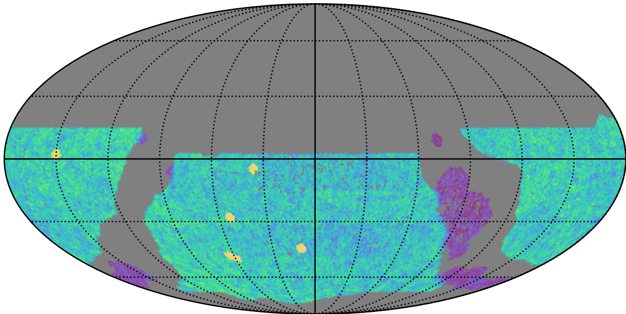
ddf_acor_sf10_lsf40_lsr10_v3.4_10yrs WFD u band: NVisits
