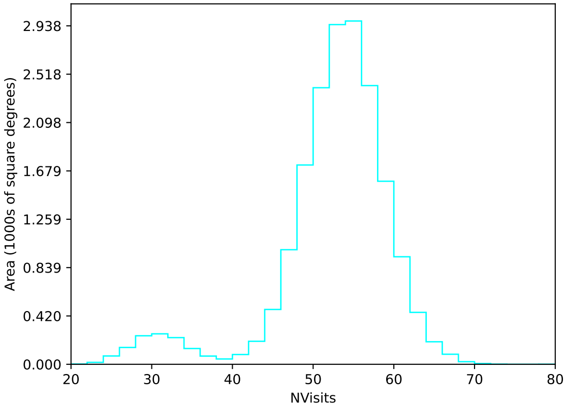
ddf_acor_sf10_lsf40_lsr10_v3.4_10yrs WFD u band: NVisits
