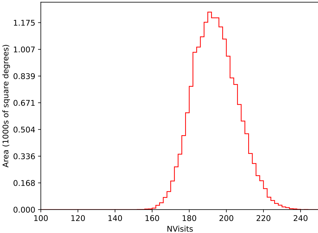
ddf_acor_sf10_lsf40_lsr10_v3.4_10yrs WFD i band: NVisits
