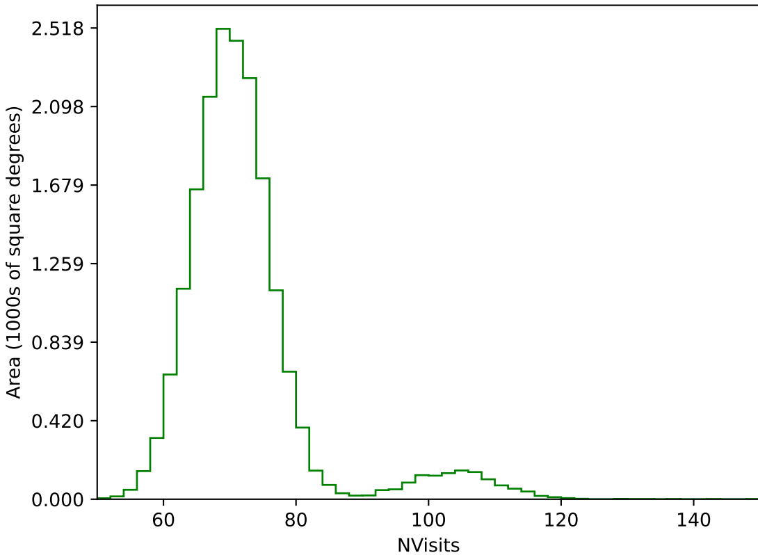
ddf_acor_sf10_lsf40_lsr10_v3.4_10yrs WFD g band: NVisits
