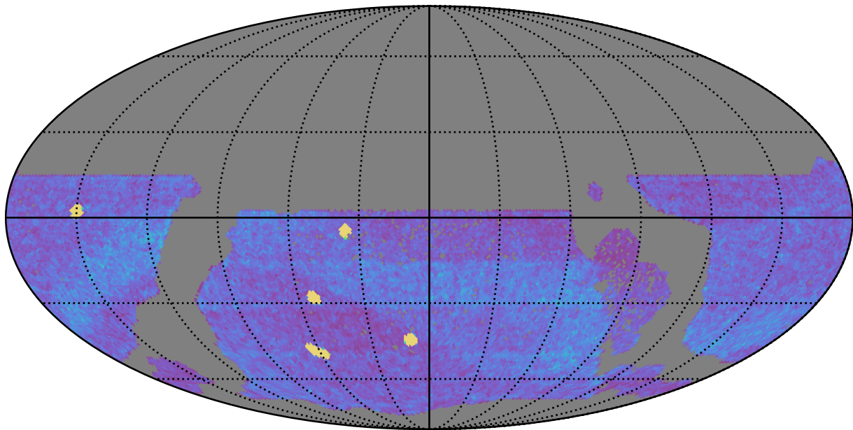
ddf_acor_sf10_lsf40_lsr10_v3.4_10yrs WFD all bands: NVisits
