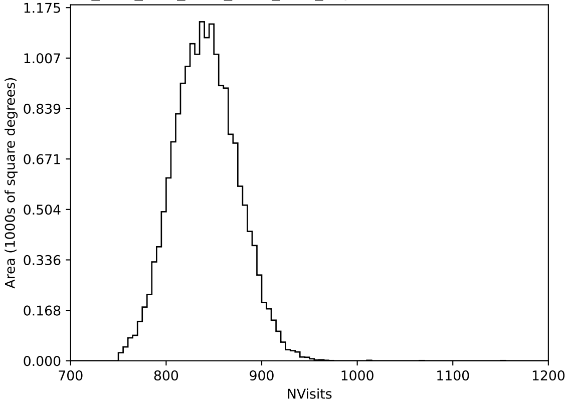
ddf_acor_sf10_ls40_lsr10_v3.4_10yrs WFD all bands: NVisits
