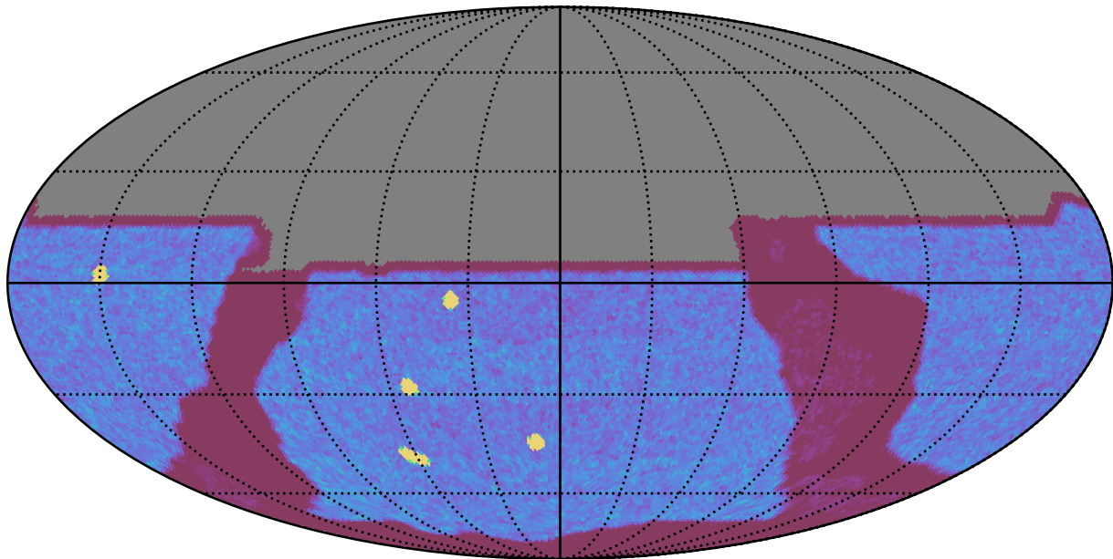
ddf_acor_sf10_lsf40_lsr10_v3.4_10yrs All sky y band: NVisits
