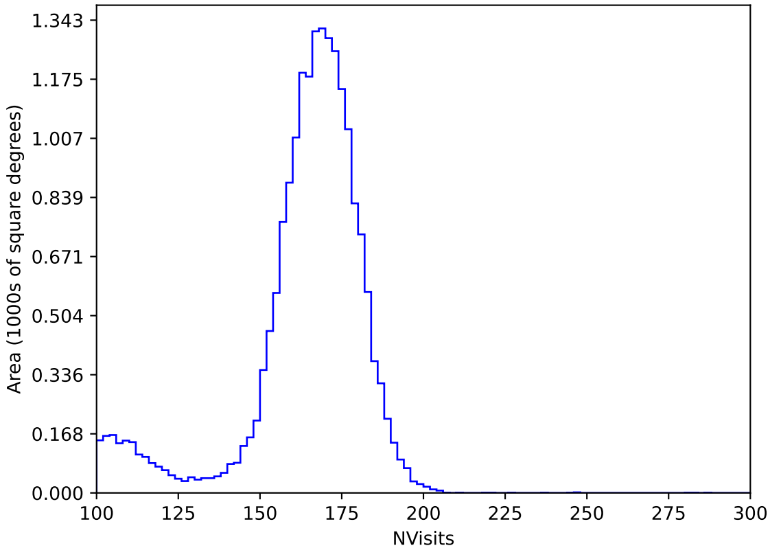
ddf_acor_sf10_lsf40_lsr10_v3.4_10yrs All sky y band: NVisits
