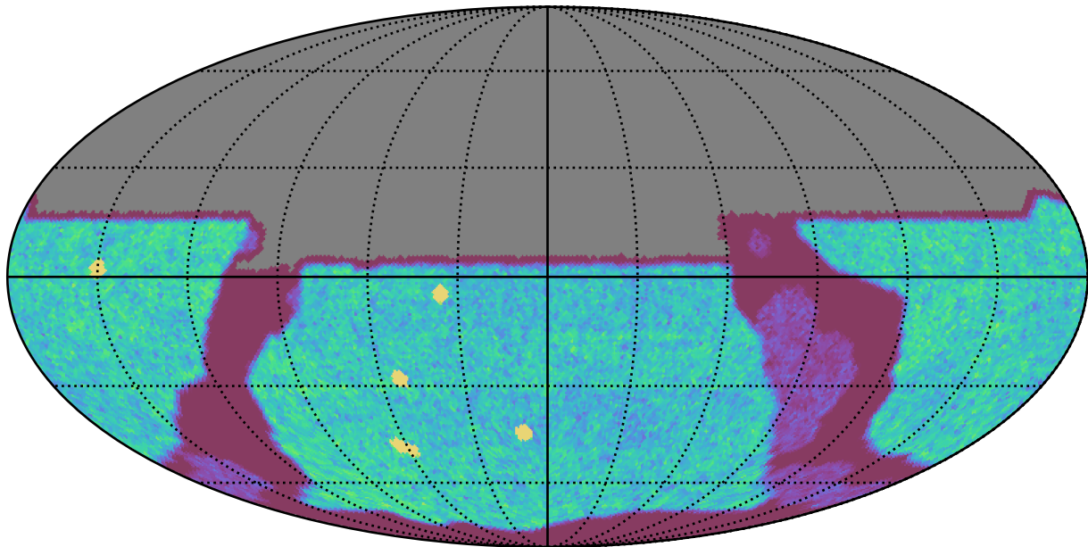
ddf_acor_sf10_lsf40_lsr10_v3.4_10yrs All sky u band: NVisits
