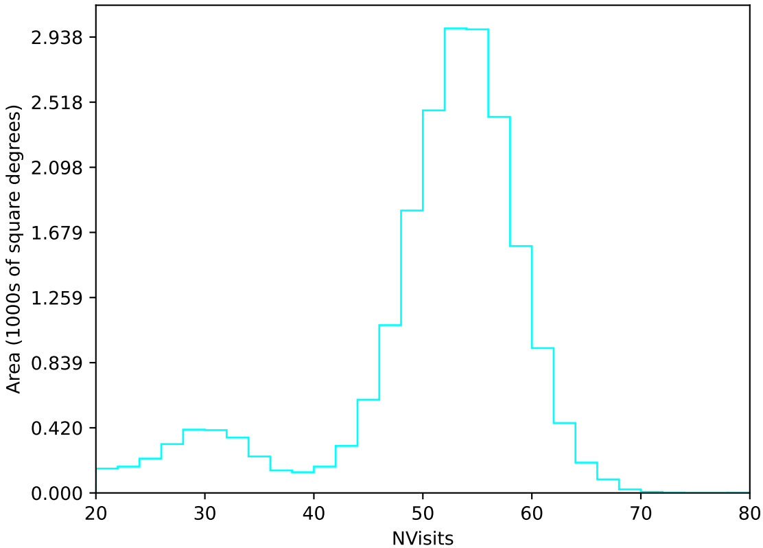
ddf_acor_sf10_lsf40_lsr10_v3.4_10yrs All sky u band: NVisits
