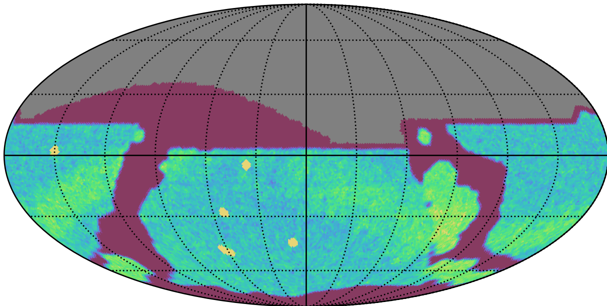
ddf_acor_sf10_lsf40_lsr10_v3.4_10yrs All sky r band: NVisits
