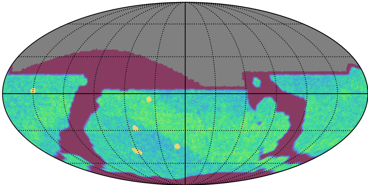
ddf_acor_sf10_lsf40_lsr10_v3.4_10yrs All sky i band: NVisits
