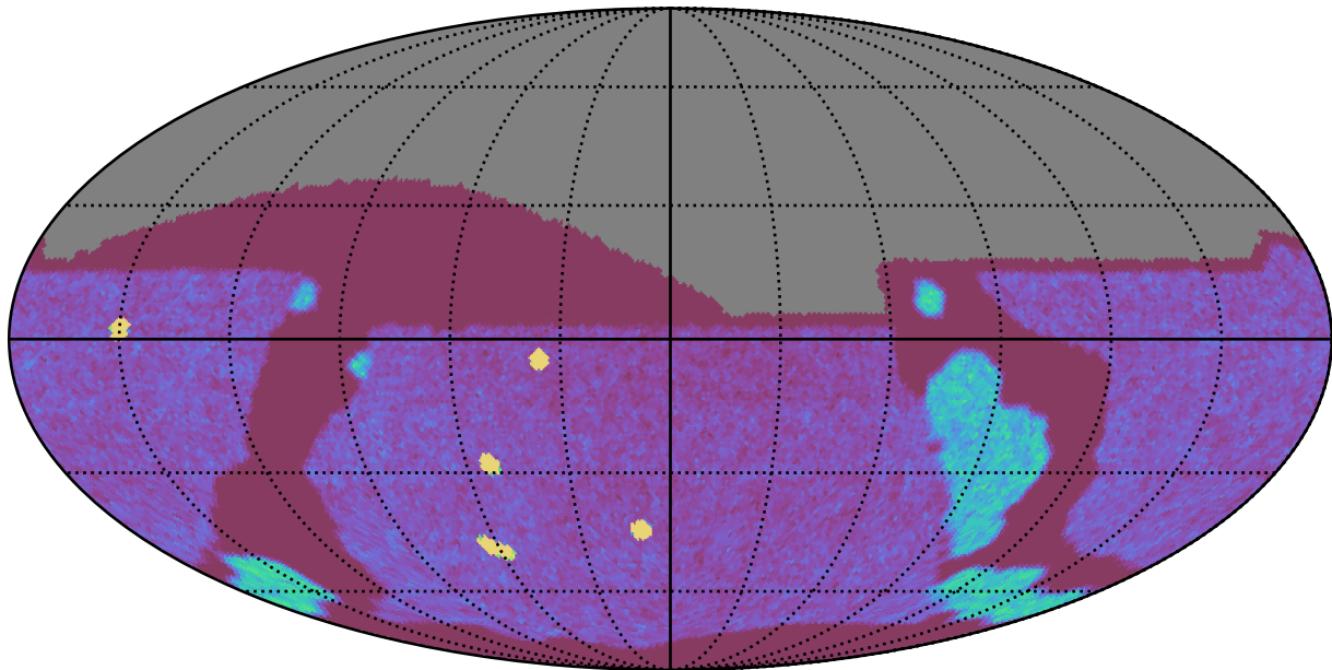
ddf_acor_sf10_lsf40_lsr10_v3.4_10yrs All sky g band: NVisits
