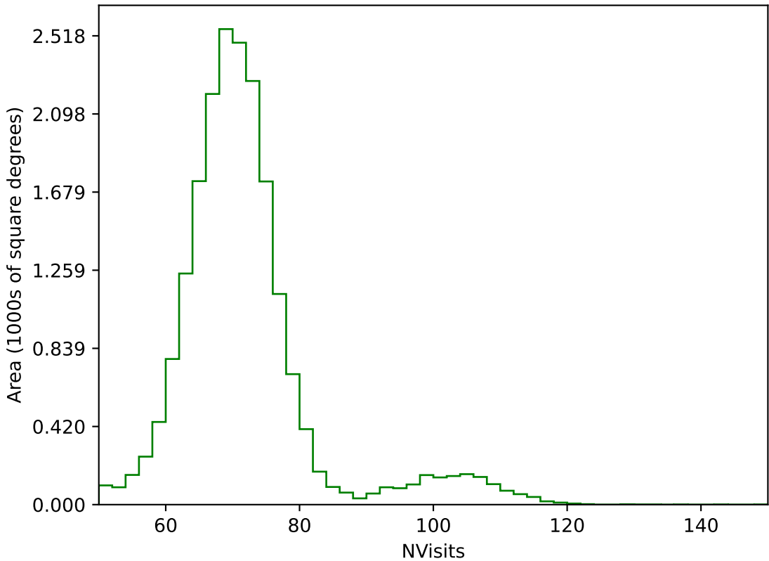
ddf_acor_sf10_lsf40_lsr10_v3.4_10yrs All sky g band: NVisits
