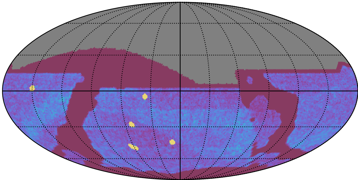
ddf_acor_sf10_lsf40_lsr10_v3.4_10yrs All sky all bands: NVisits
