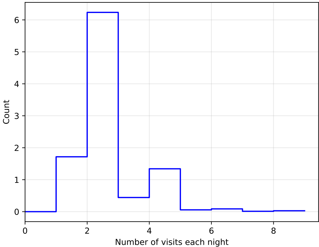
ddf_acor_sf10_lsf40_lsr10_v3.4_10yrs All sky: NVisitsPerNight 1e6
