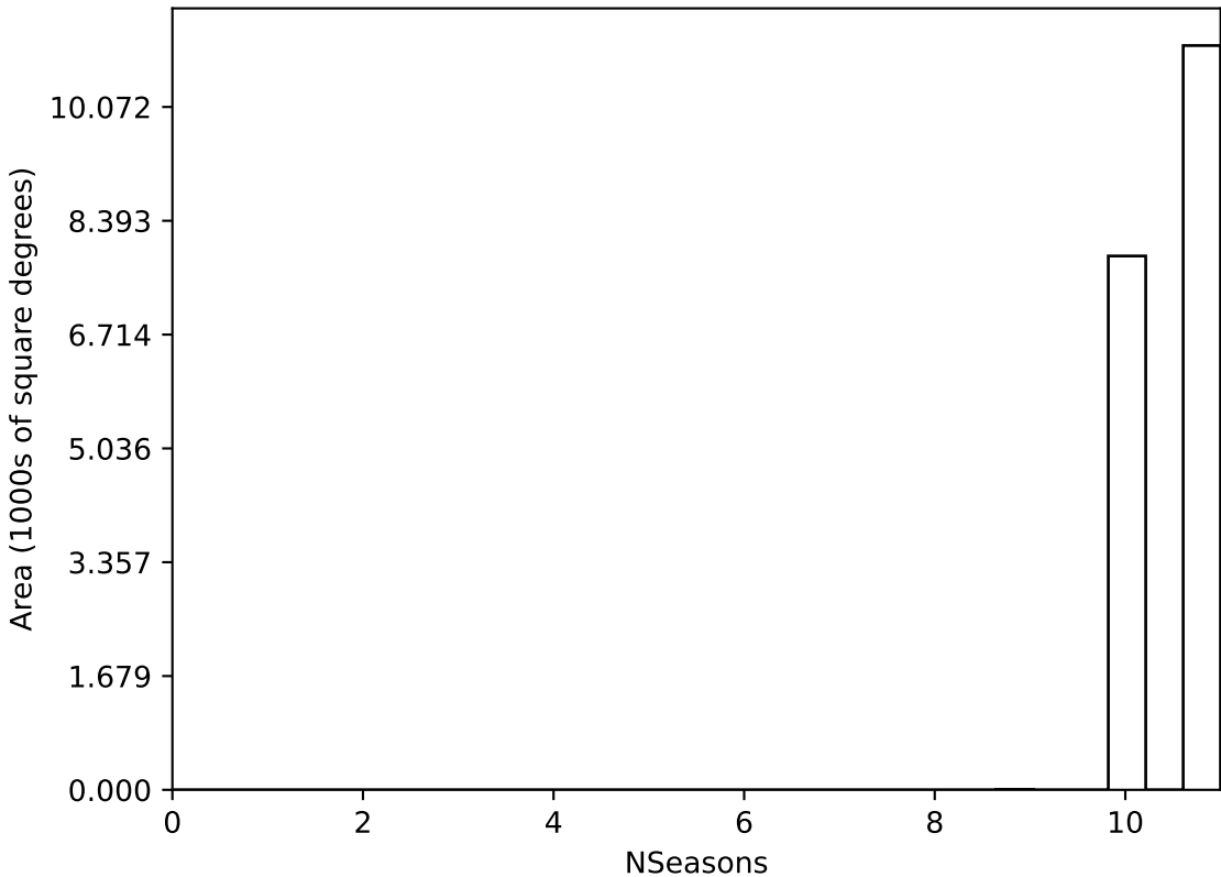
ddf_acor_sf10_lsf40_lsr10_v3.4_10yrs WFD all bands: NSeasons
