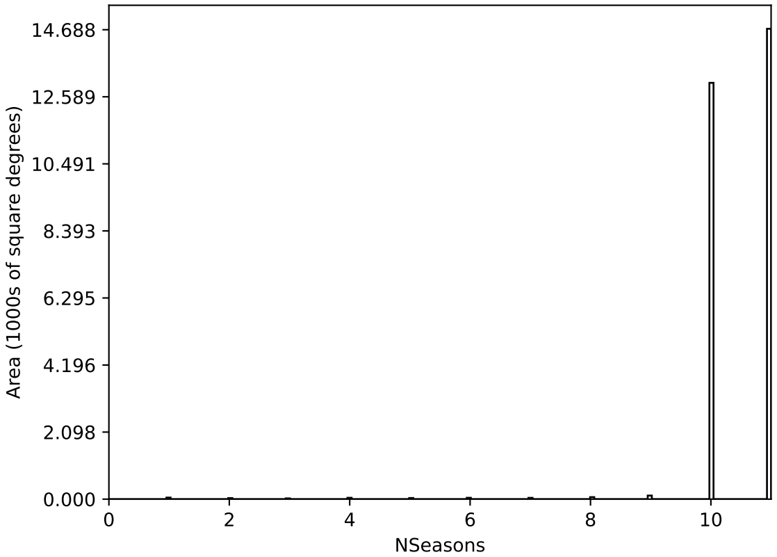
ddf_acor_sf10_lsf40_lsr10_v3.4_10yrs All sky all bands: NSeasons
